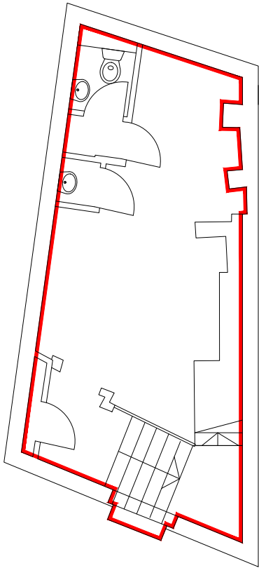
BASEMENT PLAN SCALE 1:100
